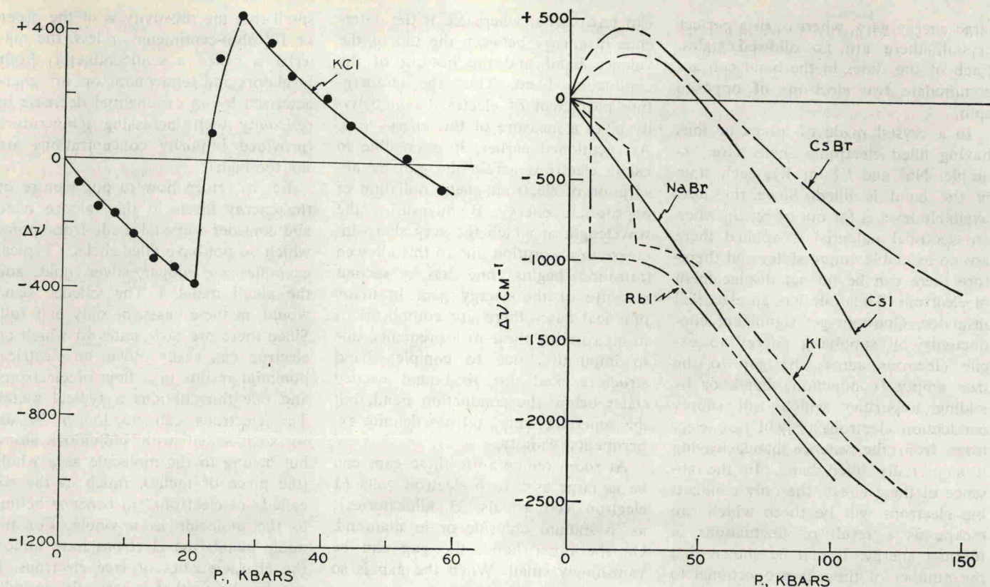
Fig. 2 (left). \Delta\nu plotted against pressure for potassium chloride with \text{TI}^+ . Fig. 3 (right). \Delta\nu plotted against pressure for \text{TI}^+ in alkali halides.
